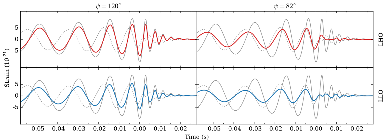
FIG. 5. Comparison of detector responses using NR waveform CFUIB0020 at an angle \theta_{IN} = 92^\circ . Incoming h_+ and h_\times polarizations are shown by grey solid and dashed curves respectively. The left column shows the theoretical detector response (Eq. (9)) in red for LHO on the top row and in blue for LLO on the bottom row, for a polarization angle of \psi = 120^\circ . The right column shows the responses for a polarization angle of \psi = 82^\circ . In both cases the distance to the source is 40 Mpc. The signal at LHO has been inverted to account for the relative detector orientations, and the signals are aligned in time; cf. Fig. 1 in [1]. We find significant differences in the detector responses between the two polarization angles (see text for details).
