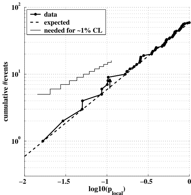
FIG. 3: Cumulative local probability distribution resulting from the search of 59 IFO-IFO on-source pairs using a 25-ms crosscorrelation length. The most significant excess is indicated by the arrow. The expected distribution under the null hypothesis is indicated by the bold, dashed line. The excess needed for a \sim 1\% confidence in the null hypothesis is indicated by the solid line. The maximum excess indicated by this line is 15 events because only the 15 most significant events in the actual distribution are tested.
