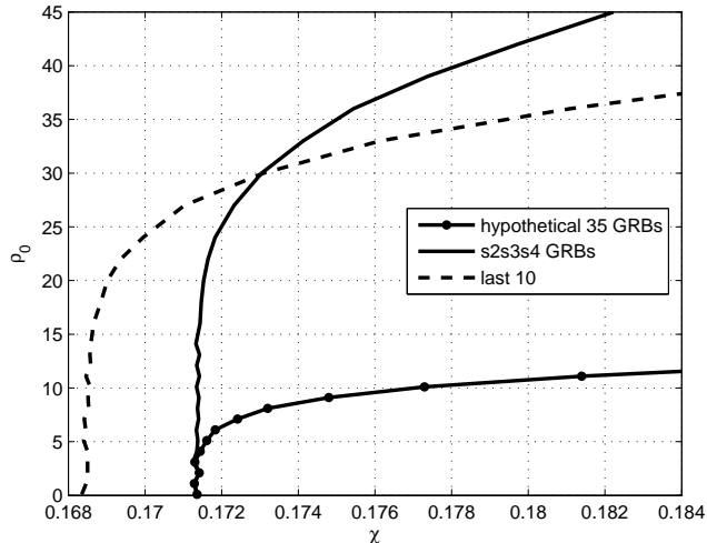
FIG. 10: Upper limit confidence belts at 90% confidence level on \rho_0 , the SNR at the most probable redshift for Swift GRBs given in [59]. The solid line is the curve for all S2, S3, S4 GRBs that were used in the H1-H2 search (on-source \chi = 0.1753 ). The dashed line is the curve when only the last 10 GRBs from the above set are selected (on-source \chi = 0.1702 ). The line with filled circles is for a hypothetical scenario with 35 GRBs, all with an optimal sky location, and two identical and constant sensitivity detectors. The shifting of the curves horizontally is due to the change in the variance of \chi as the number of GRBs is changed. For each value of \rho_0 , 10,000 values of \chi were drawn from its marginal distribution.
