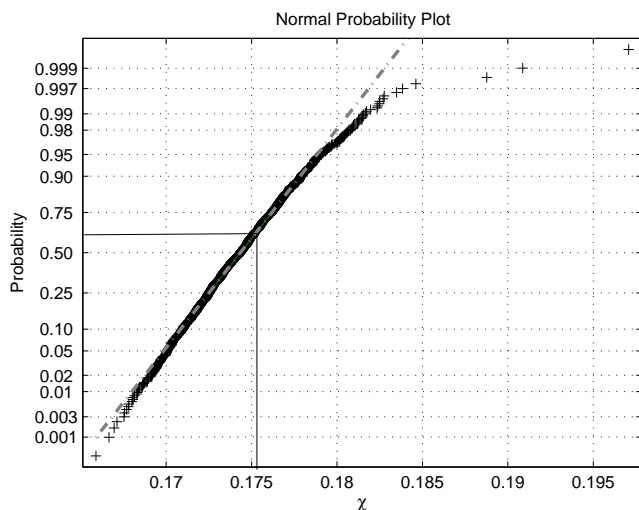
FIG. 6: Plot of the cumulative distribution function of the off-source values of the sum-max statistic \chi . The dashed line shows the best fit normal distribution. The solid horizontal and vertical lines indicate the location of the on-source values of \chi_{\text{on}} and the corresponding cumulative probability. The on-source value was \chi_{\text{on}} = 0.1753 , which yields a cumulative probability of 0.64 or an empirical significance of 1 - 0.64 = 0.36 .
