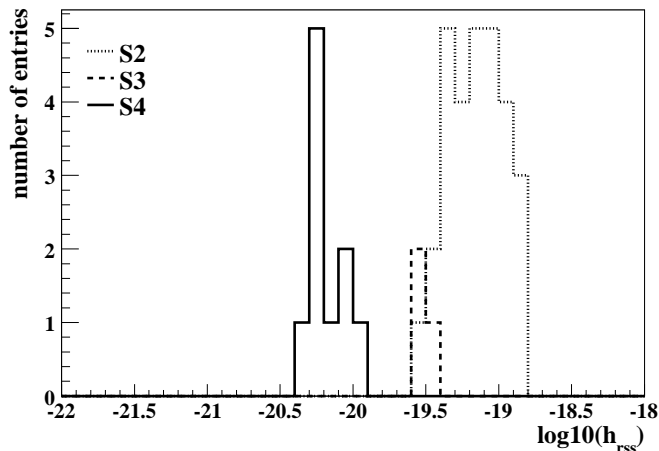
FIG. 8: Progression of h_{\text{rss}} upper limits from the S2 to S4 LIGO runs for linearly polarized sine-gaussian waveforms; 25-ms crosscorrelation.
