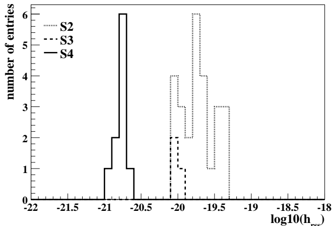
FIG. 9: Progression of h_{\text{rss}} upper limits from the S2 to S4 LIGO runs for circularly polarized sine-gaussian waveforms; 25-ms crosscorrelation.
