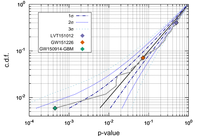
Figure 4. Cumulative distribution function of empirically-determined of p -values for the targeted search. The black solid line corresponds to the null hypothesis that the search sample is consistent with background. The blue dashed lines envelop the 1-, 2-, and 3- \sigma confidence intervals. The highest ranking (lowest p -value) event is GW150914-GBM (green diamond) which, for this search, has a significance of \gtrsim 1.5\sigma .
